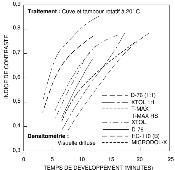
Courbes d'indice de contraste Film KODAK PROFESSIONAL TRI-X 320 / 320TX 120/220
